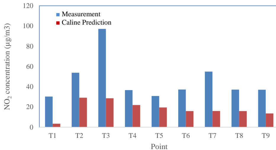
Figure 7. Comparison of pollutant concentrations of nitrogen dioxide ( \text{NO}_2 )
