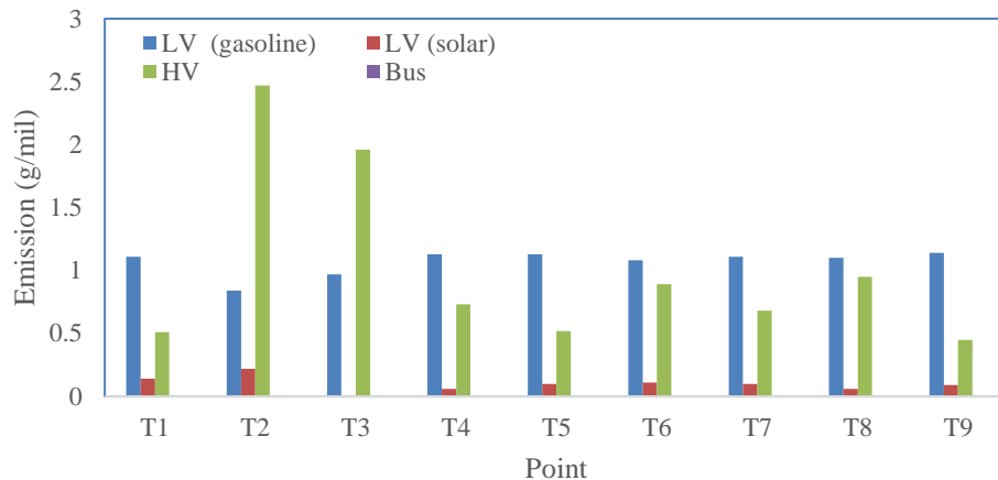
Figure 3. NO 2 emissions by type of vehicle
